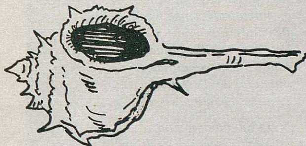
Murex Brandaris
